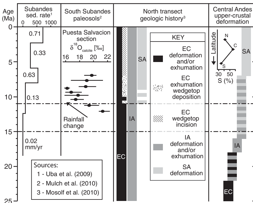
Figure 3. Geologic data consistent with enhanced rainfall starting 15–11 Ma (dashed lines); sed—sedimentation, S—shortening. Transects: N—north, C—center, S—south; AL—Altiplano, EC—Eastern Cordillera, IA—Interandean zone, SA—Subandes. See text for discussion. Central Andes deformation history is integrated over all transects plus data from Peru and Argentina (Espurt et al., 2011). Inset is latitudinal variations in SA shortening with 5% error (McQuarrie, 2002; McQuarrie et al., 2008a).
