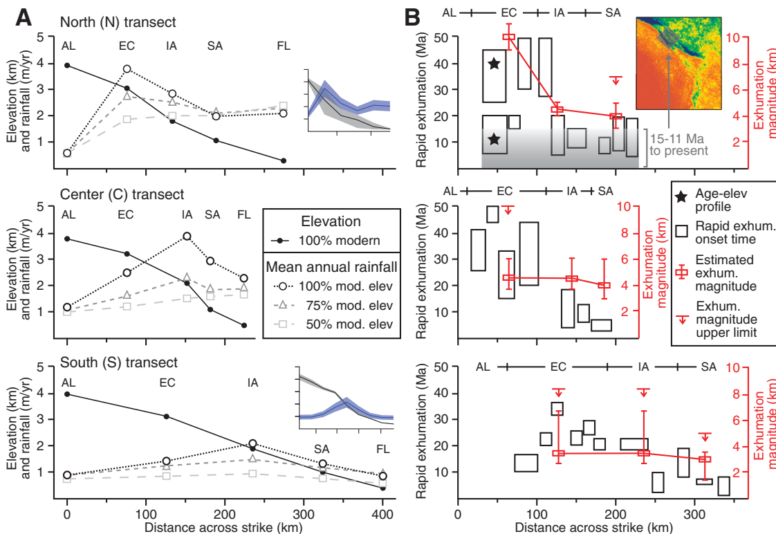
Figure 2. Climate and exhumation along transects in Figure 1. A: Regional circulation model REMO iso rainfall estimates for 50%, 75%, and 100% modern (mod) elevations (elev) compared to 100% model elevations. Insets are ~150 km swath profiles for 100% mod elevation run for comparison to Figure 1B profiles. B: Cordilleran exhumation patterns (Fig. 1A data). Gray is rapid exhumation (exhum.) since ca. 15–11 Ma that correlates with climate in north. Inset is spatial extent overlying Tropical Rainfall Measuring Mission (TRMM) rainfall (Fig. 1B). Stars are best age constraints (age-elevation profiles) for both exhumation phases in the northern EC (Gillis et al., 2006).
